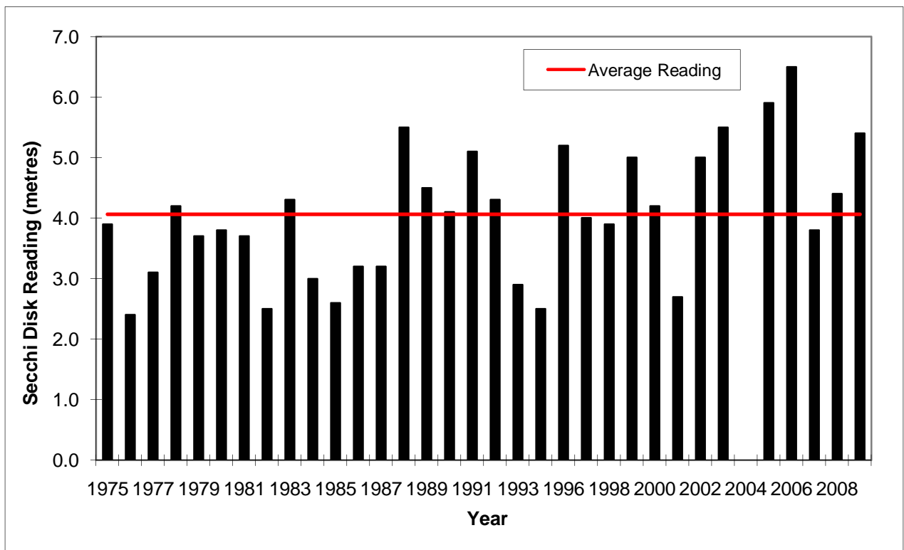
Figure 1: Pike Lake Average Annual Water Clarity Based on Secchi Disk Depth
