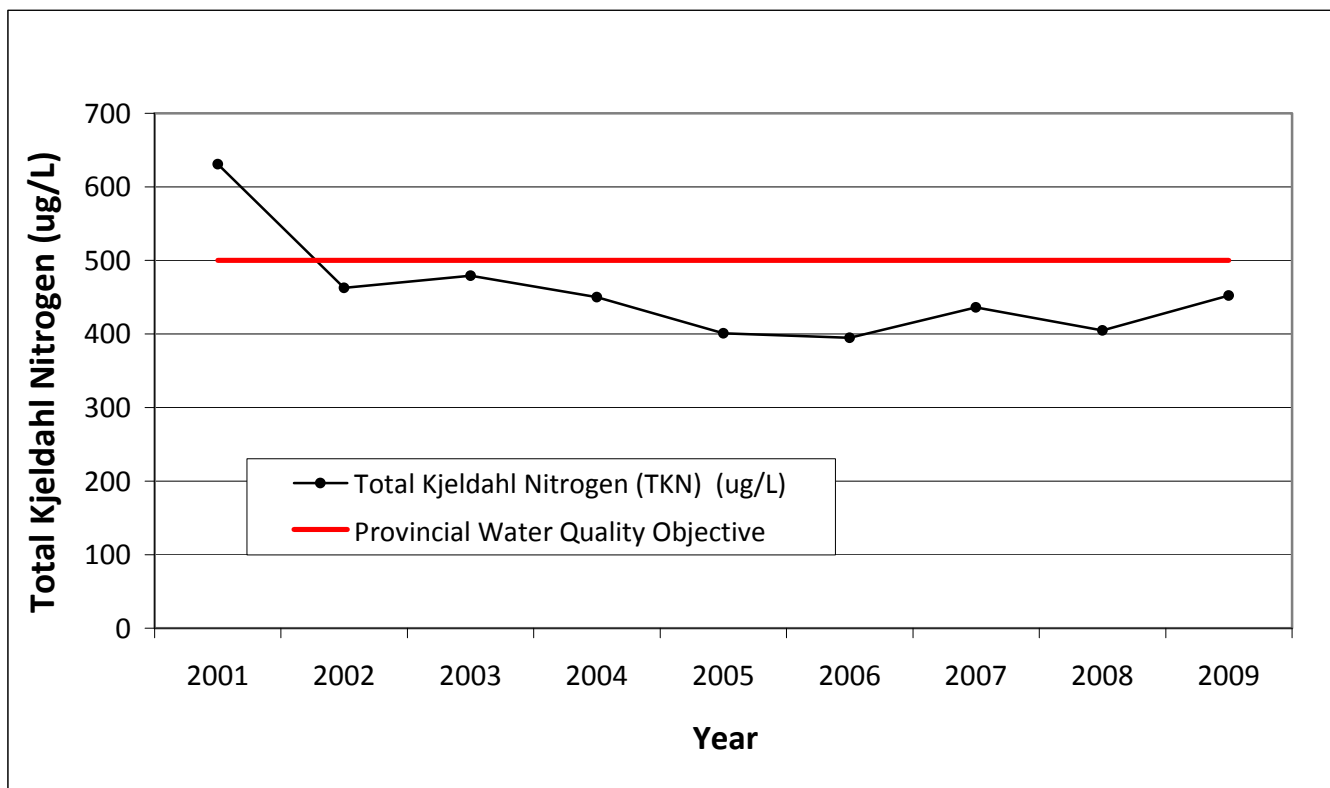
Figure 5: Yearly Average Total Kjeldahl Nitrogen on Pike Lake (2001 - 2009)
