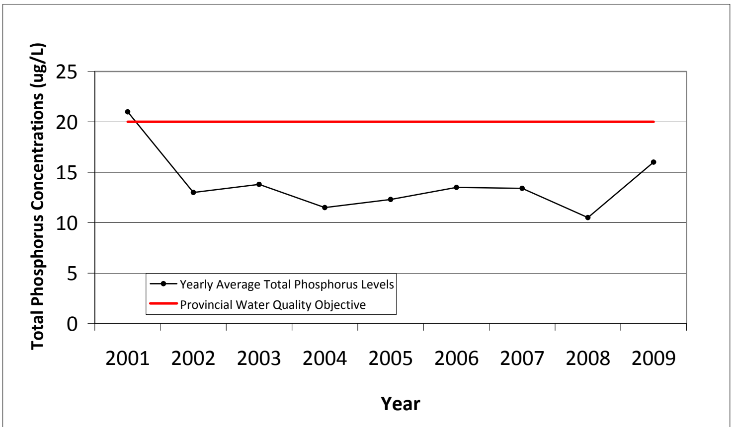
Figure 4: Yearly Average Total Phosphorus on Pike Lake (2001 - 2009)
